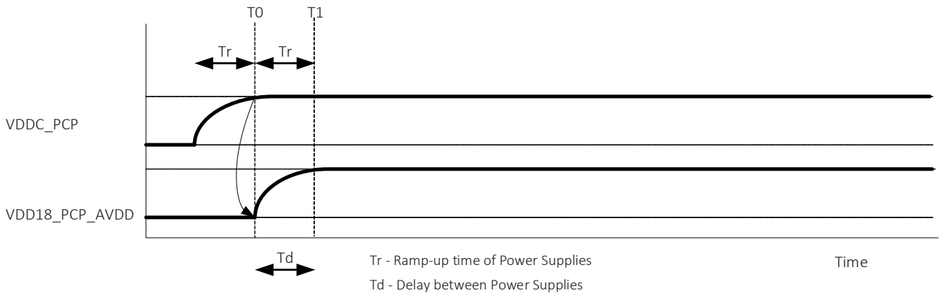
Figure 5: Power-on Voltage Sequencing – PCP Domain
