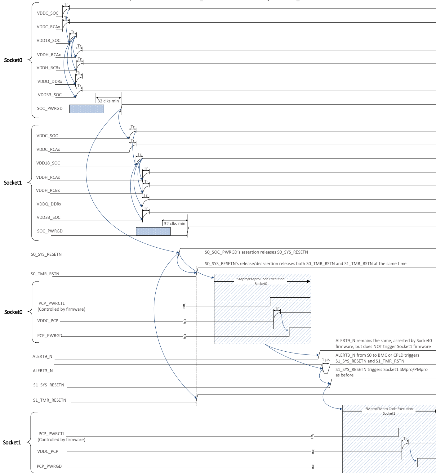
Figure 9: Power-on Sequence for 2P Configuration when ALERT9_N is Not Connected to CPLD
